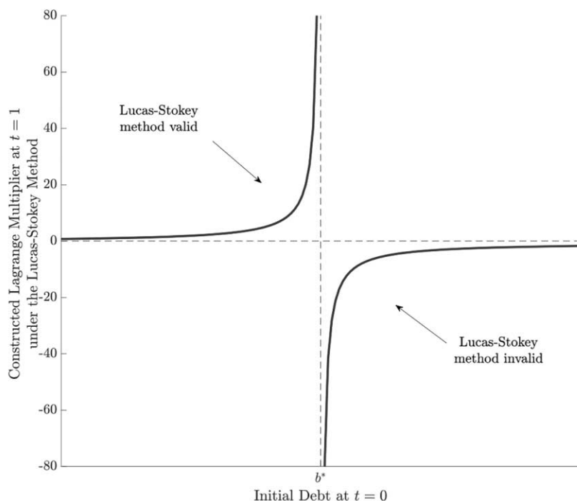
FIG. 4.—Initial debt and constructed Lagrange multiplier. The x-axis shows the initial debt at t = 0 , b . The y-axis shows the constructed Lagrange multiplier under the Lucas-Stokey method, \lambda_1 . We set \eta = \gamma = 1 , g = 0.2 , and \beta = 0.5 . The value of b^* is the level of debt above which optimal policy sets date 1 taxes above the peak of the Laffer curve. A color version of this figure is available online.
