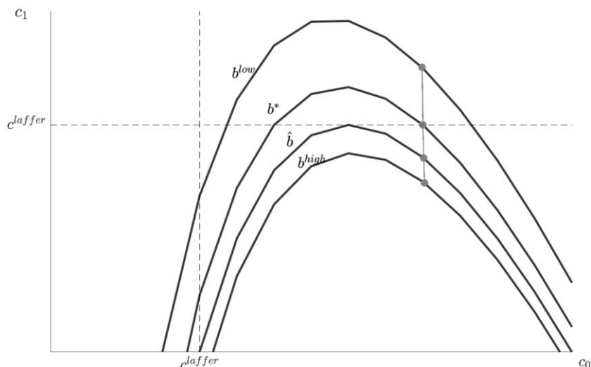
FIG. 2.—Implementable allocations and optimal policy. Solid black lines denote the combinations of \{c_0, c_1\} that satisfy the implementability condition for different levels of initial debt b^{low} < b^* < \hat{b} < b^{high} . Filled circles correspond to optimal policies. We set \eta = \gamma = 1 , g = 0.2 , and \beta = 0.5 . The value of c^{laffer} is the level of consumption associated with the peak of the Laffer curve. The value of b^* is the level of debt above which optimal policy sets date 1 taxes above the peak of the Laffer curve, even though setting taxes below the peak may satisfy the implementability condition. The value of \hat{b} is the level of debt above which optimal policy sets date 1 taxes above the peak of the Laffer curve because setting taxes below the peak of the Laffer curve cannot satisfy the implementability condition. A color version of this figure is available online.
