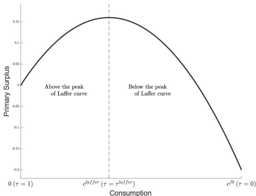
FIG. 1.—Primary surplus and consumption. This figure depicts the primary surplus, \tau n - g , as a function of consumption, c . We set \eta = \gamma = 1 and g = 0.2 . The figure refers to the common representation of the curve as revenue \tau n as a function of the tax rate \tau . The values of \tau^{laffer} and c^{laffer} are the tax rate and level of consumption associated with the peak of the Laffer curve, respectively. The value of c^{fb} is the level of consumption associated with the first best. The region below the peak of the Laffer curve corresponds to the case where \tau < \tau^{laffer} , and the region above the peak of the Laffer curve corresponds to the case where \tau > \tau^{laffer} . A color version of this figure is available online.
