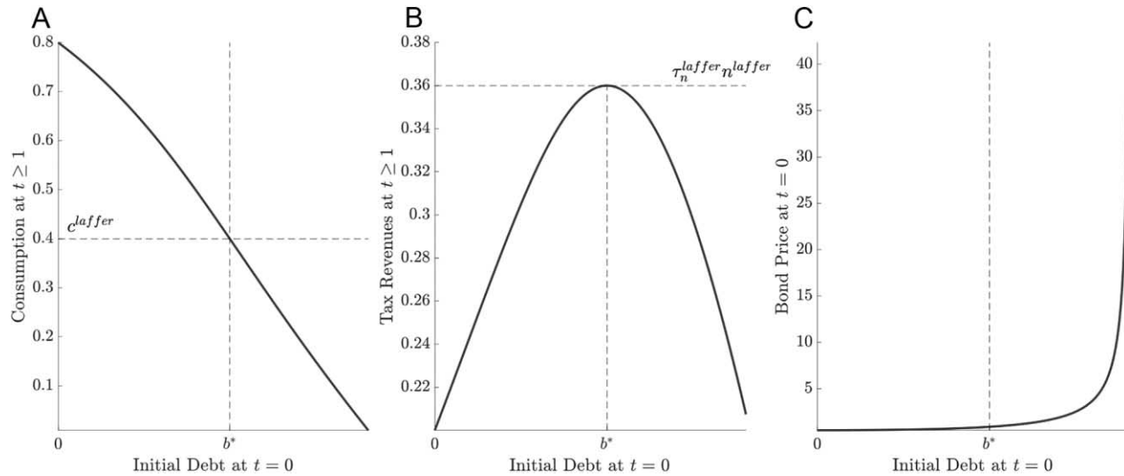
FIG. 3.—Initial debt and optimal policy. The x-axis in all panels shows the initial debt at t = 0 , b . The y-axis in A shows consumption from t = 1 onward, c_1 . The y-axis in B shows revenue from t = 1 onward, \tau_1 n_1 . The y-axis in C shows the bond price at t = 0 , q_0 = \beta c_0 / c_1 . We set \eta = \gamma = 1 , g = 0.2 , and \beta = 0.5 . The value of c^{laffer} is the level of consumption associated with the peak of the Laffer curve. The value of \tau_n^{laffer} n^{laffer} is the maximal tax revenue at the peak of the Laffer curve. The value of b^* is the level of debt above which optimal policy sets date 1 taxes above the peak of the Laffer curve. A color version of this figure is available online.
