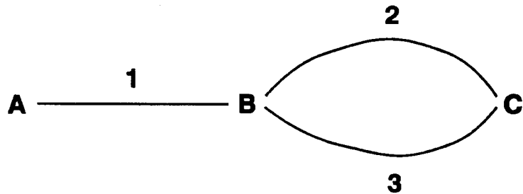
Figure 11: AB is a bottleneck facility.
