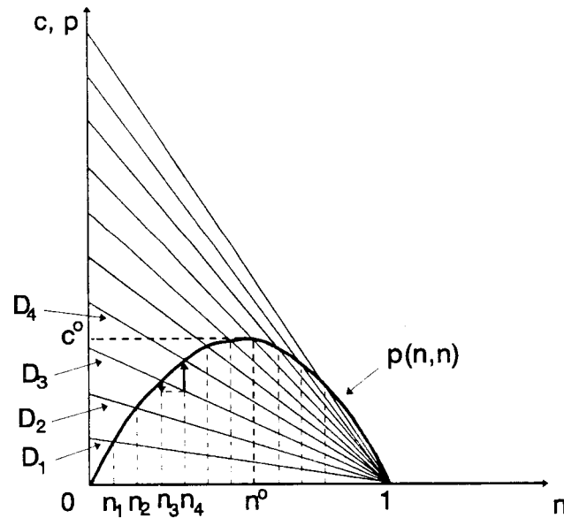
Figure 5: Construction of the fulfilled expectations demand.
