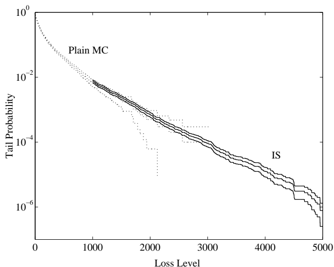
Figure 1: Comparison of plain Monte Carlo simulation (using 10,000 replications) with importance sampling (using 1,000 replications) in estimating loss probabilities in a 10-factor model. In each case, the three curves show the mean and a 95% confidence interval for each point.
