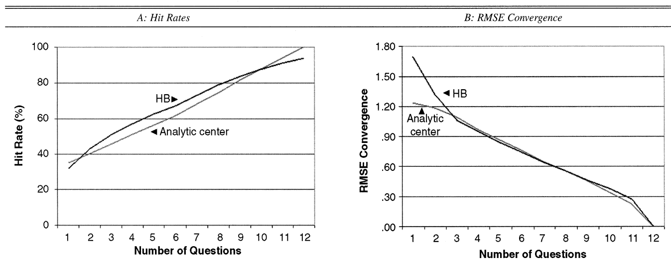
Figure 6 EMPIRICAL HIT RATES AND RMSE CONVERGENCE FOR EXECUTIVE EDUCATION STUDY
