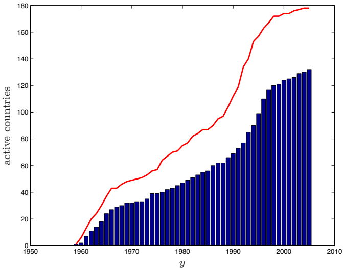
Figure 6: Degree of Germany (bars) compared vs. number of active countries |N_y| (line) for y \in \{1959, \dots, 2005\} .
