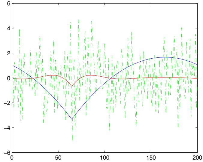
Figure 2: The pure jump signal, combined signal and noisy observations.
