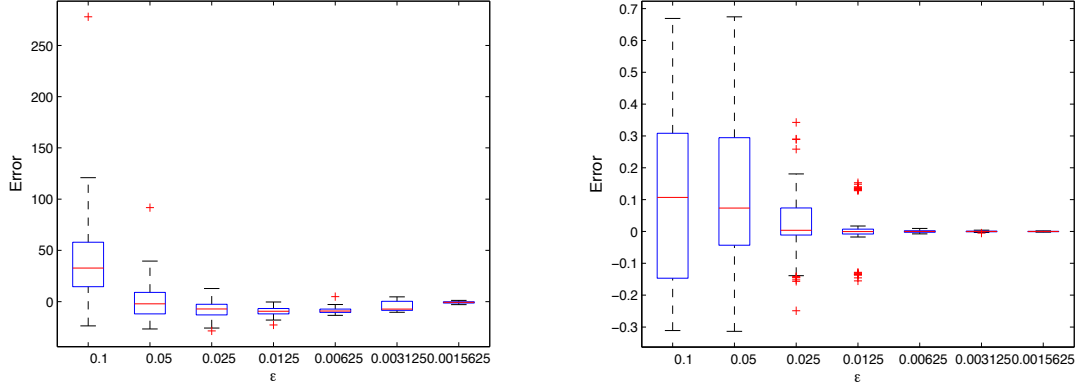
Figure 4: Boxplot of the error \hat{a}_\epsilon - |a| (left) and that of \hat{\theta}_\epsilon - \theta (right) as a function of \epsilon .
