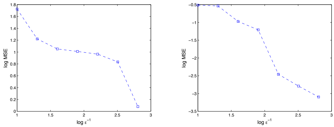
Figure 3: The log of the MSE of the estimator \hat{a}_\epsilon (left) and that of the estimator \hat{\theta}_\epsilon (right) as a function of \log \epsilon^{-1} .
